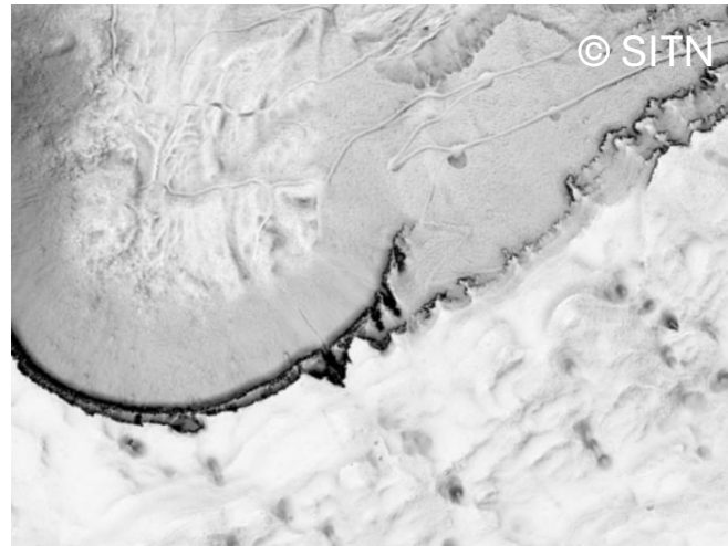
Terrain Rugdness Index
