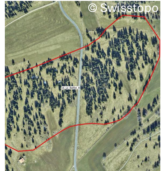
Trees spatial distribution
